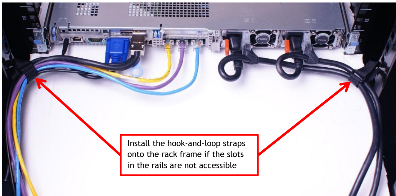
Figure 11. Cabling a system installed in static rails
