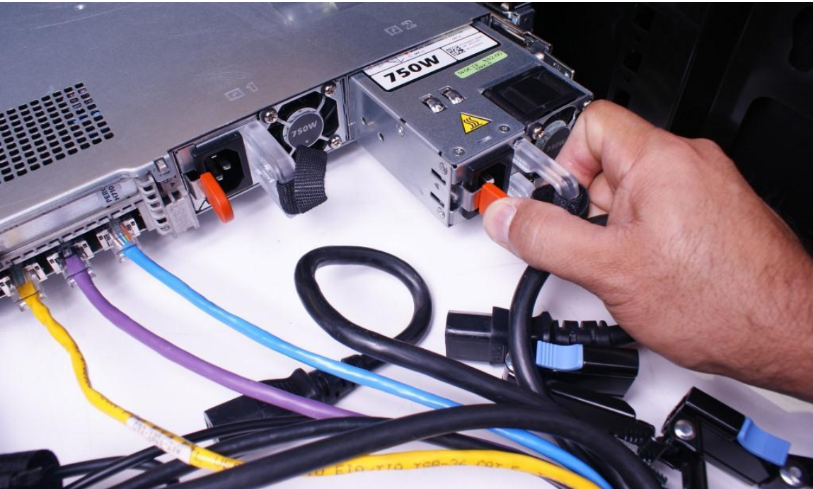
Figure 8. Replacing the outer power supply
