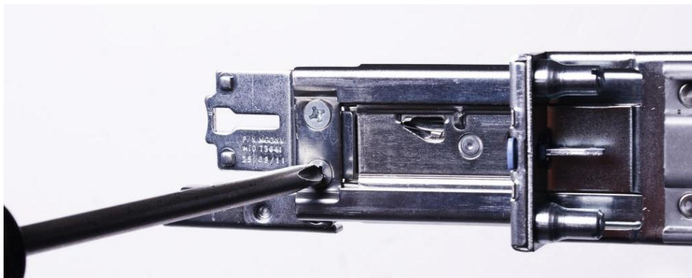
Figure 10. Removing the outer CMA brackets for shallow racks
